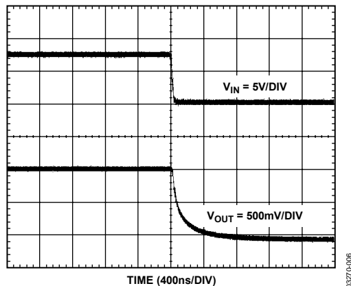
Figure 6. Turn-Off Time
